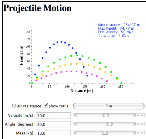
Figure 2. Projectile Motion (Fowler, 1998)
